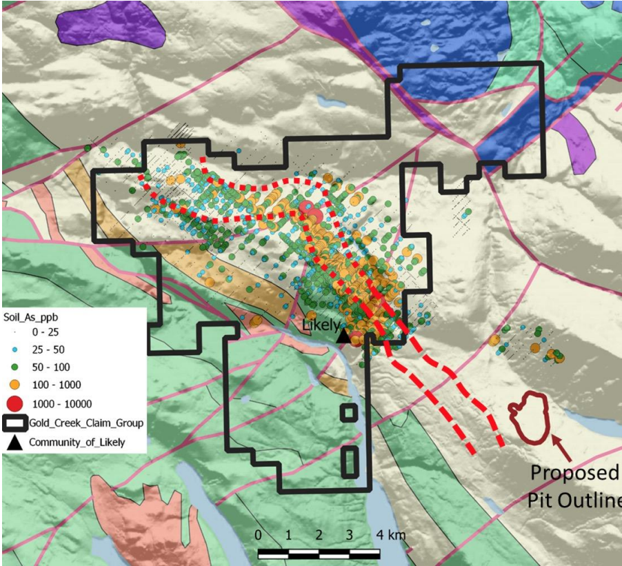
ARSENIC IN SOIL
