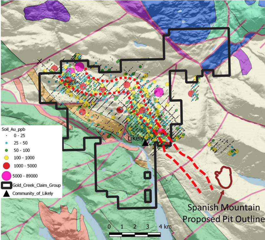
GOLD IN SOIL
