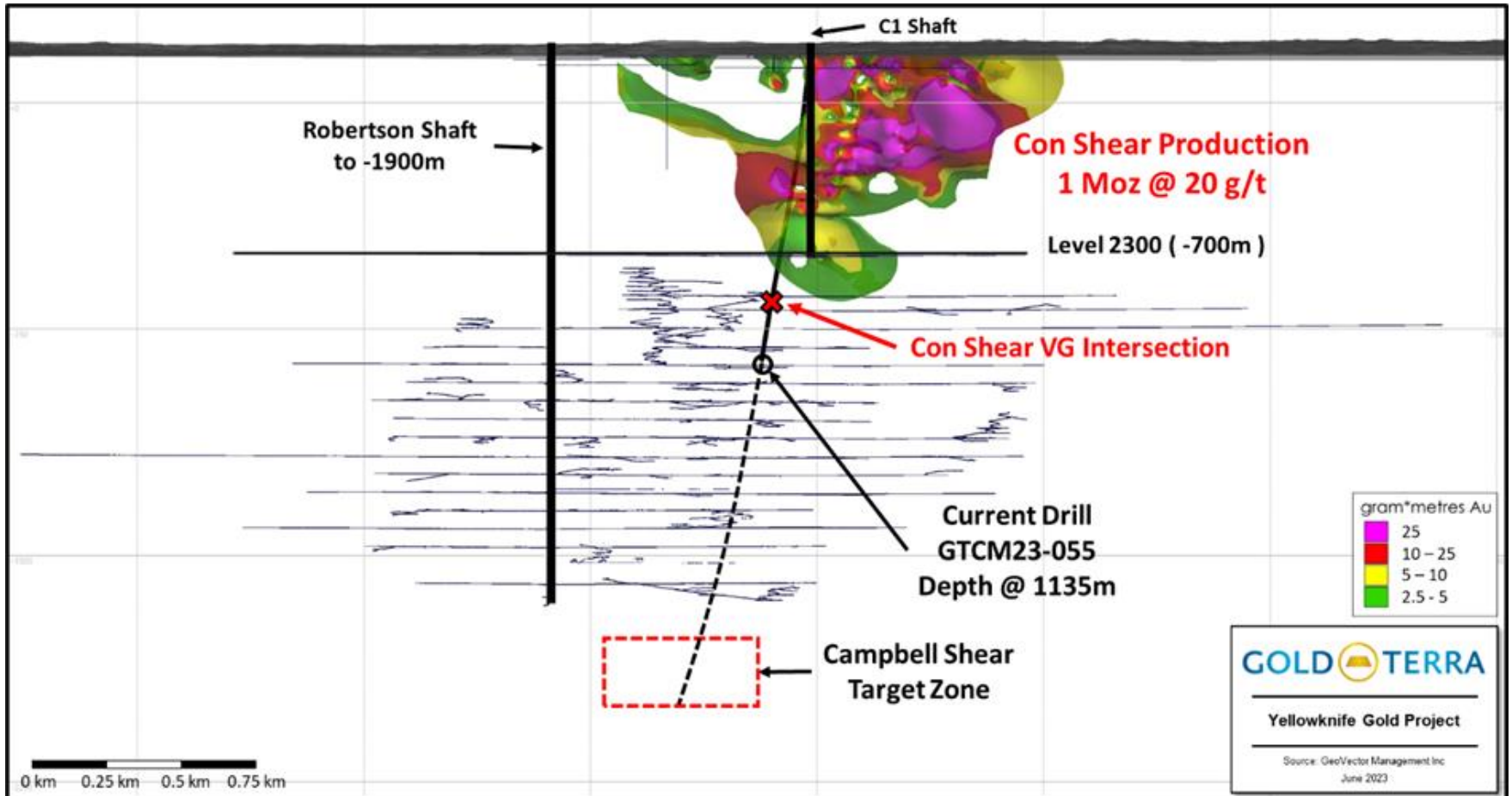
Long section looking West
