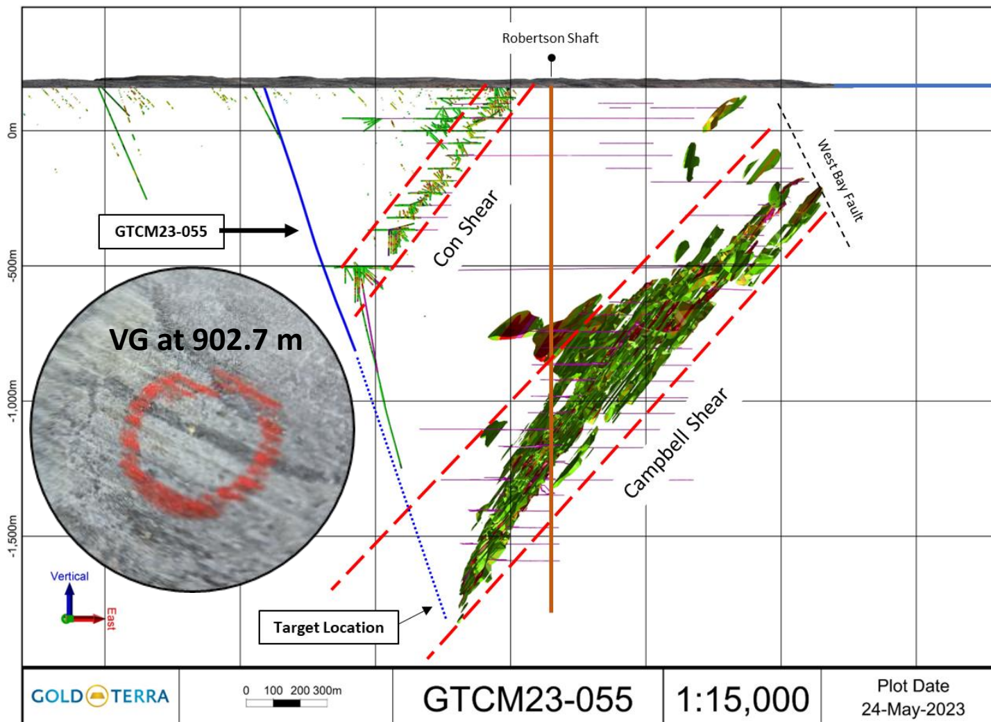
Cross-section looking North
